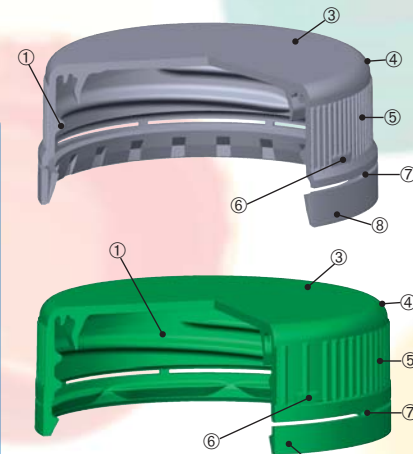
① Threads ② Liner ③ Shell ④ Side Wall ⑤ Serrations ⑥ Pull-Up Marks ⑦ Bridges ⑧ Tamper Band
